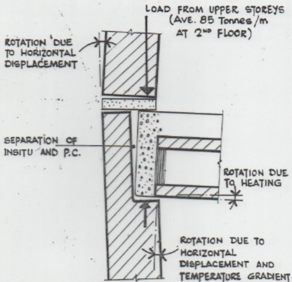
DETAIL A GEOMETRIC DISPLACEMENTS AT JOINTS
