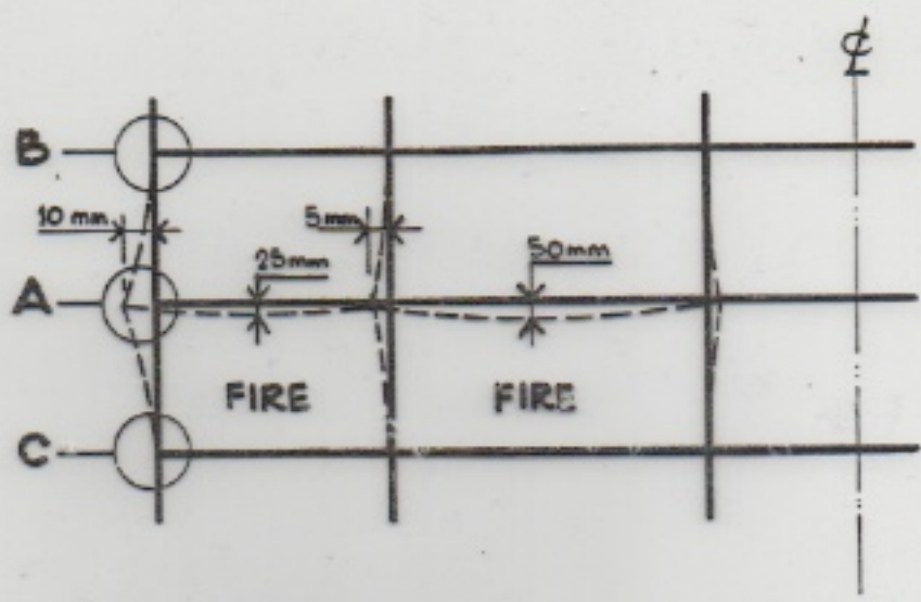
MOVEMENTS DUE TO FIRE (TWO ROOMS)
