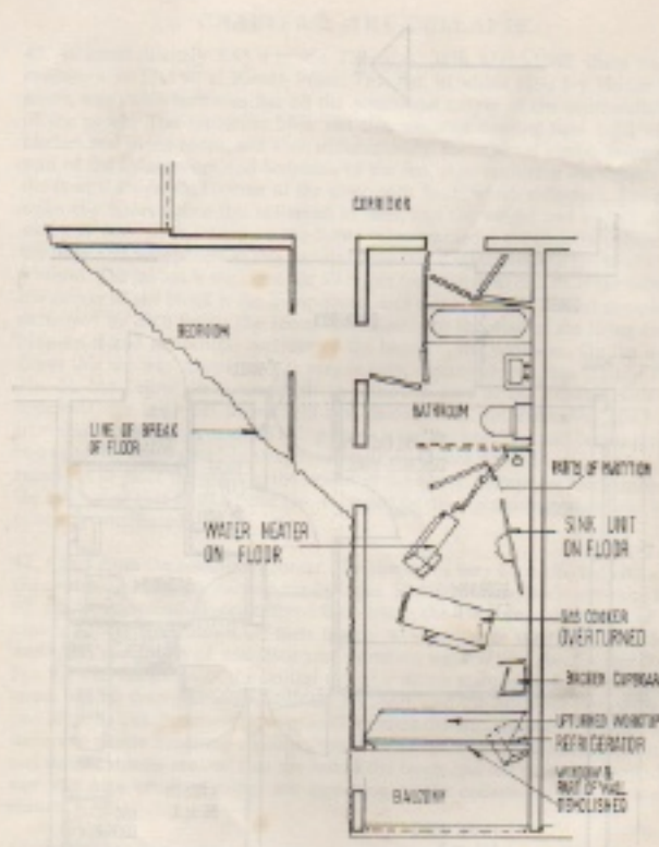
Plan (a) The extent of the damage to Flat 40
