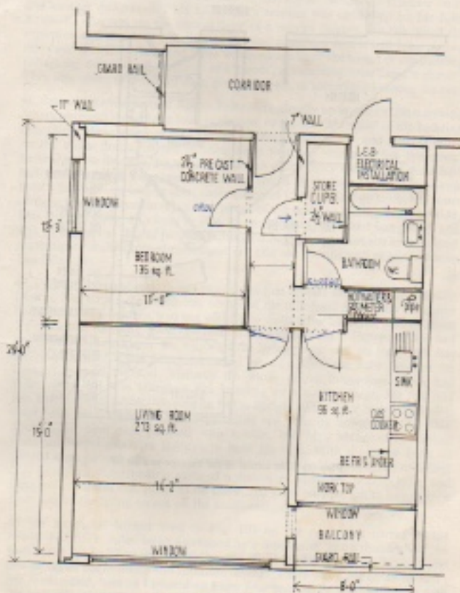
Plan (b) Layout of Flat 90
